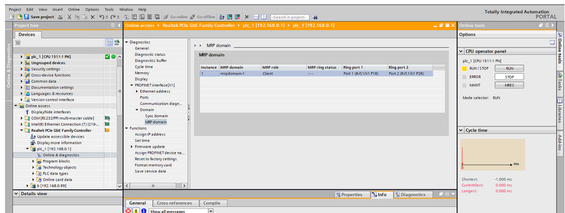
Figure 9: Define PROFINET MRP Client and MRP Domain
