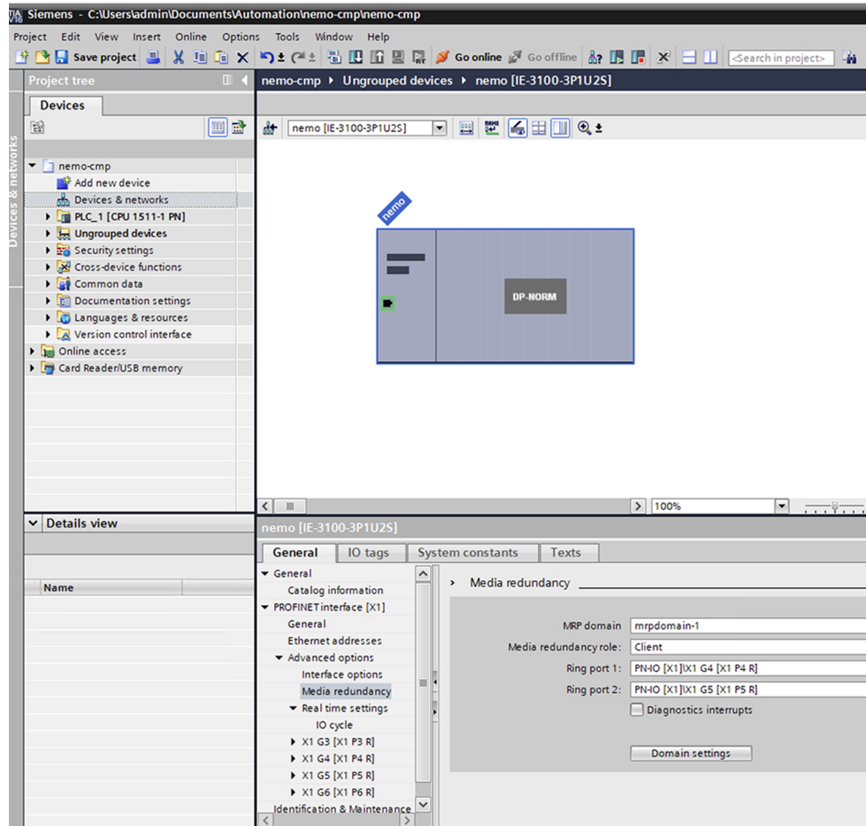
Figure 5: PROFINET MRP interfaces
