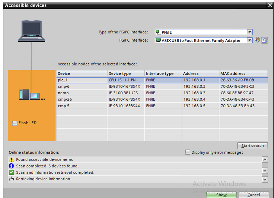
Figure 2: PROFINET Device Discovery (DCP) window before configuring MRP
