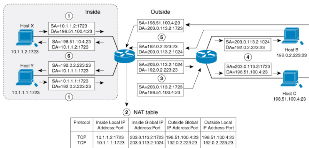
Figure 3: PAT / NAT Overloading Inside Global Addresses
