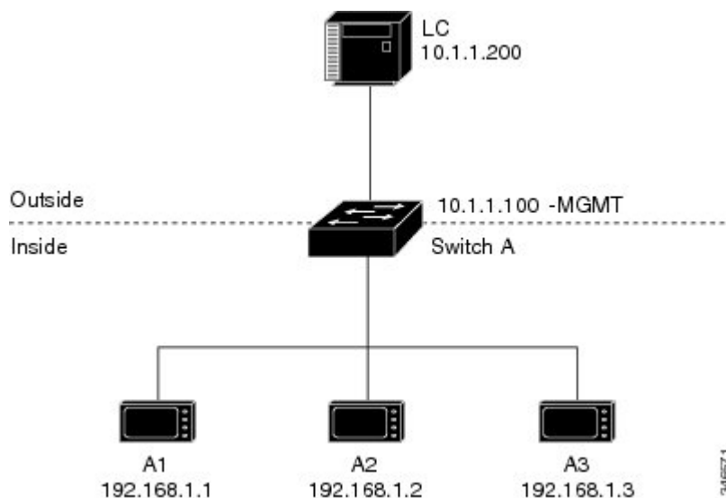
Figure 2: Basic inside-to-outside communications
