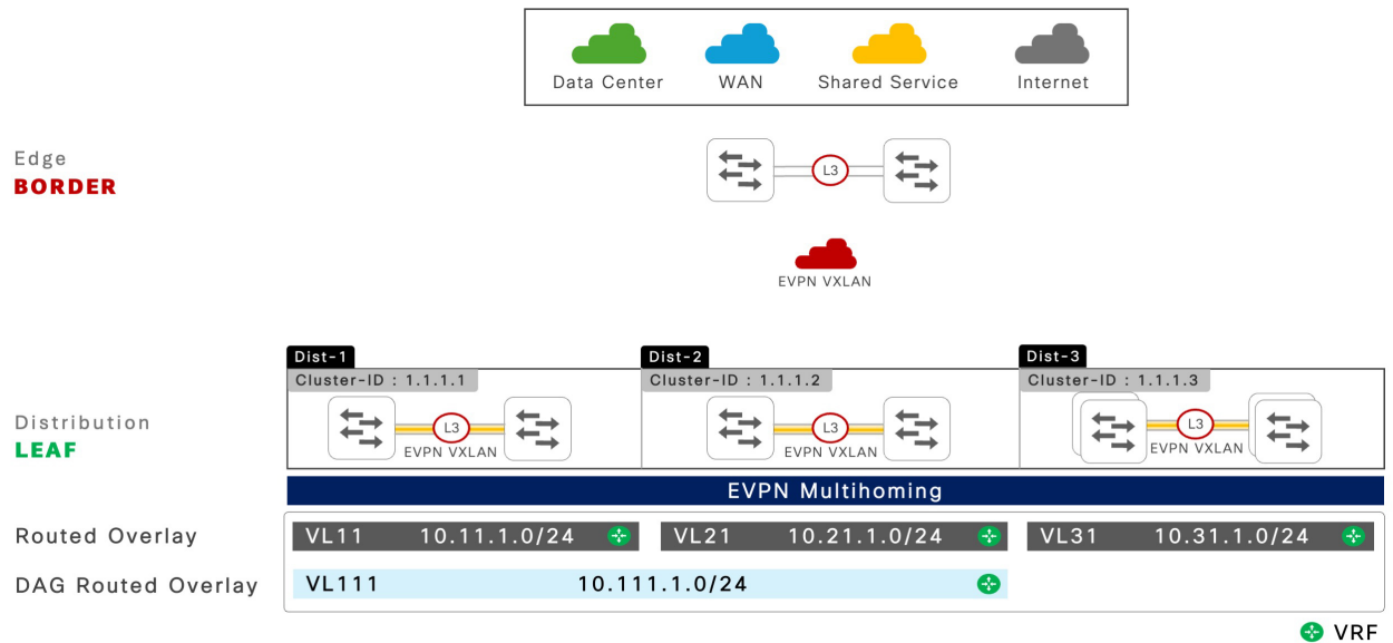
Figure 1: EVPN multihoming with DAG-routed overlay fabric network
