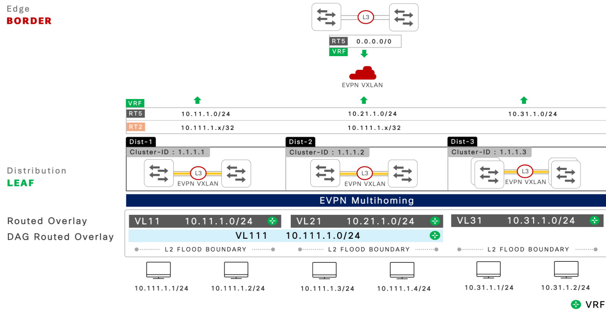
Figure 2: Key network characteristics of a DAG-routed overlay fabric
