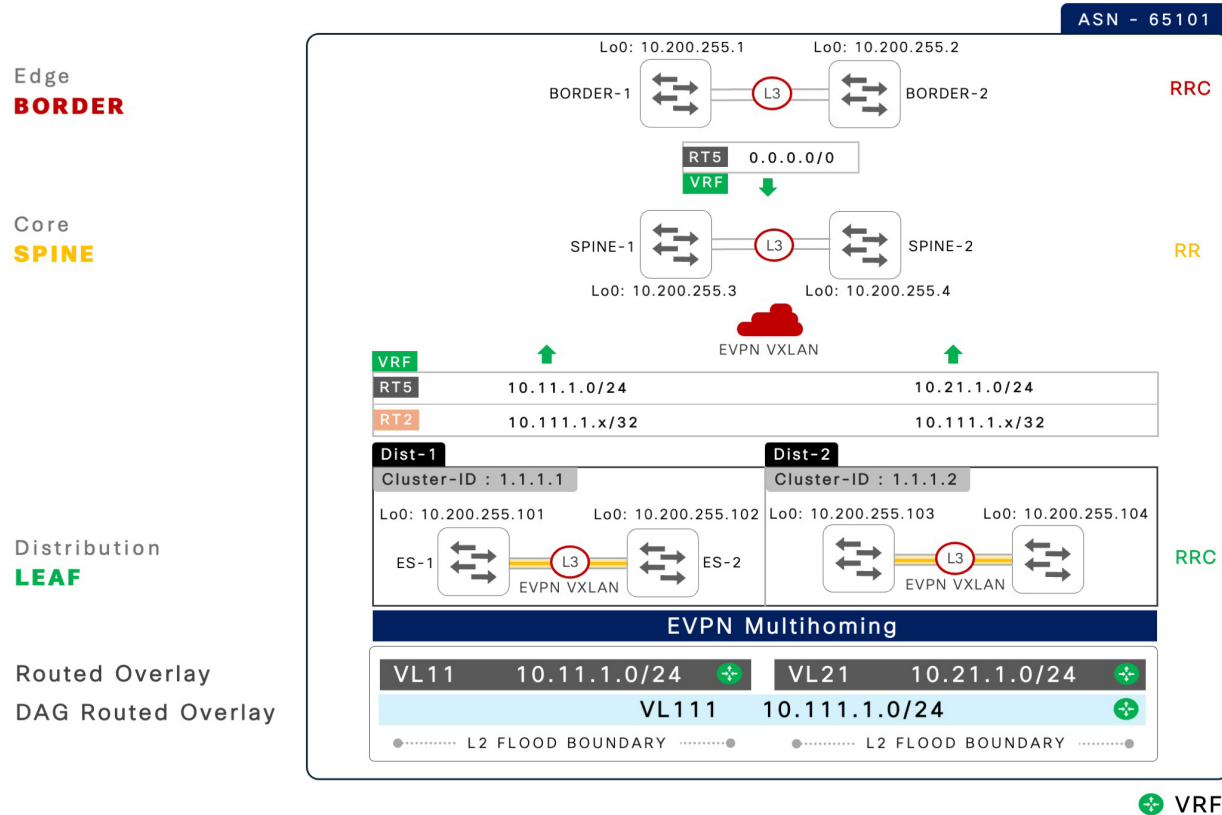
Figure 3: EVPN multihoming: DAG routed overlay fabric network
