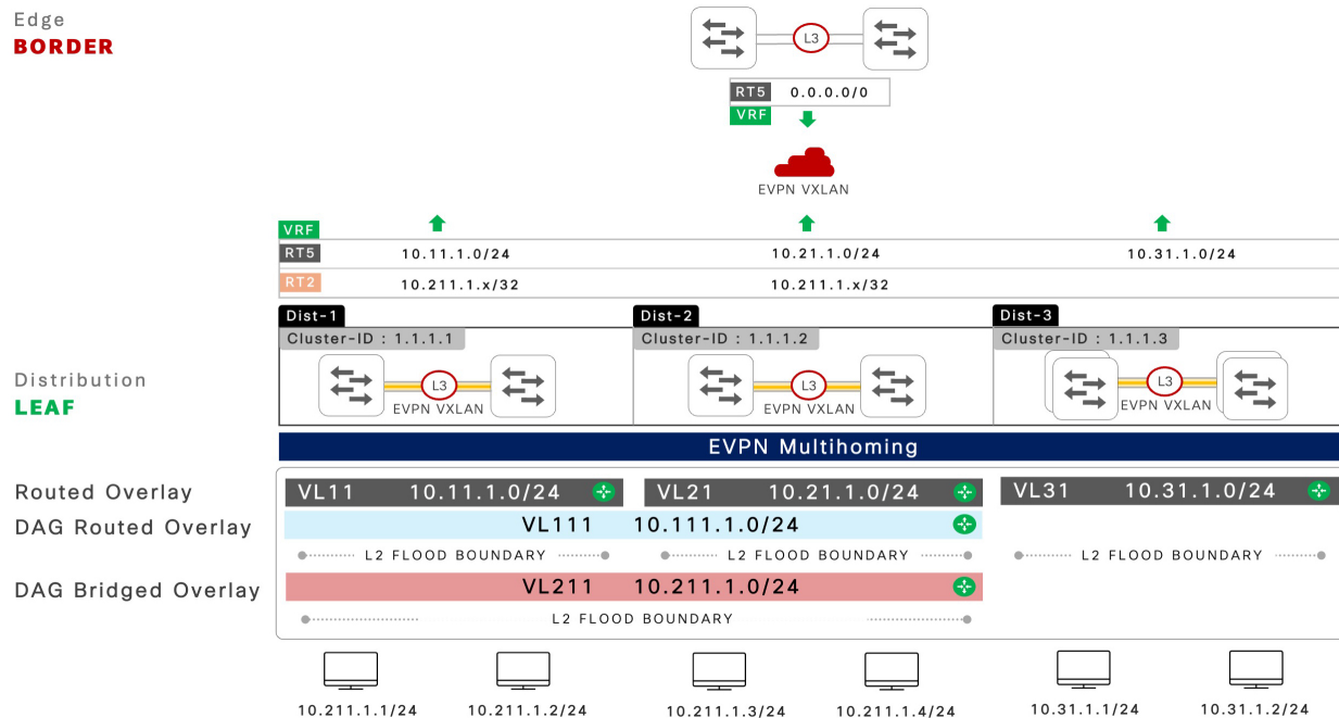
Figure 2: Key characteristics of a DAG bridged fabric overlay network
