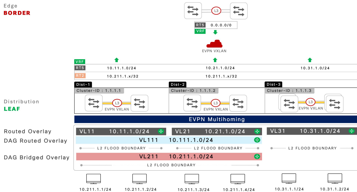
Figure 3: EVPN multihoming: DAG-brided overlay fabric network
