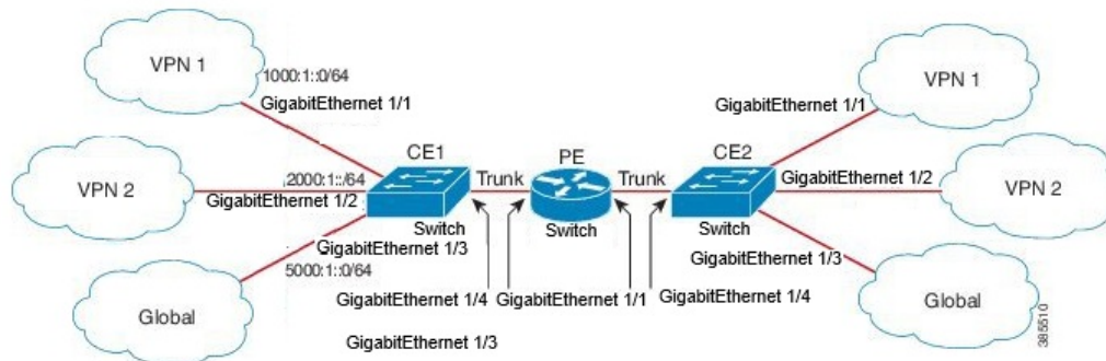
Figure 1: VRF-lite Configuration Example
