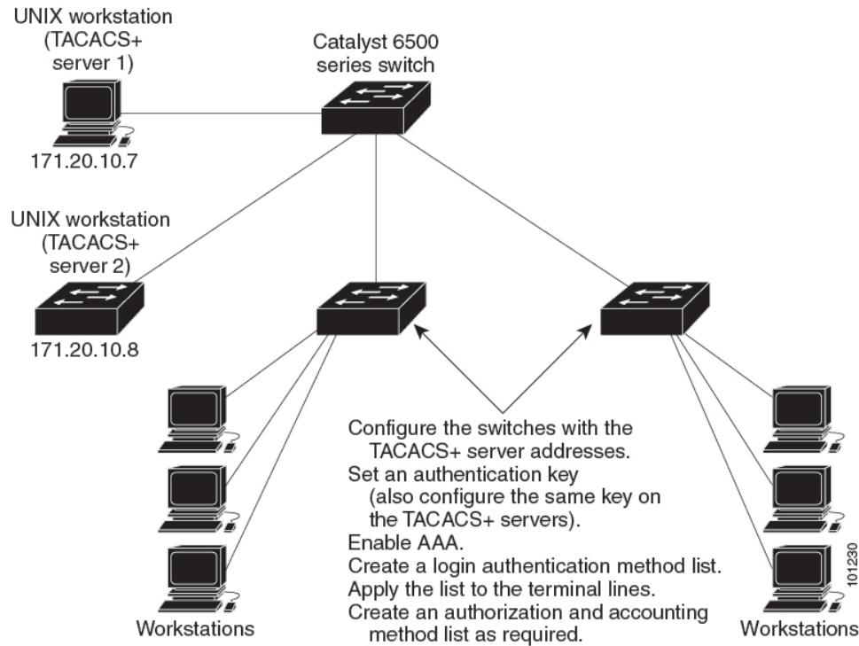
Figure 1: Network Configuration of Typical TACACS+
