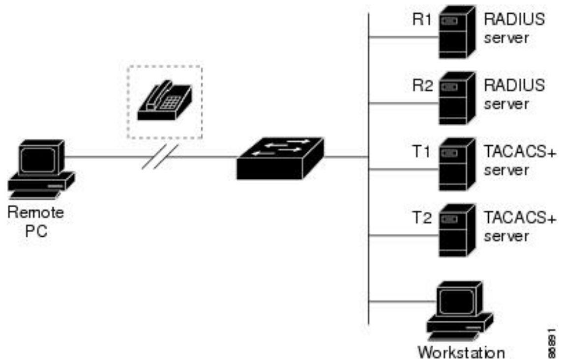
Figure 1: Transitioning from RADIUS to TACACS+ Services
