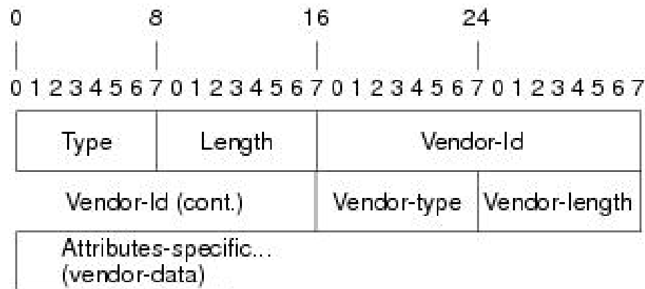
Figure 2: VSA Encapsulated Behind Attribute 26
