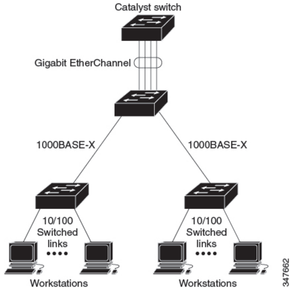
Figure 1: Typical EtherChannel Configuration
