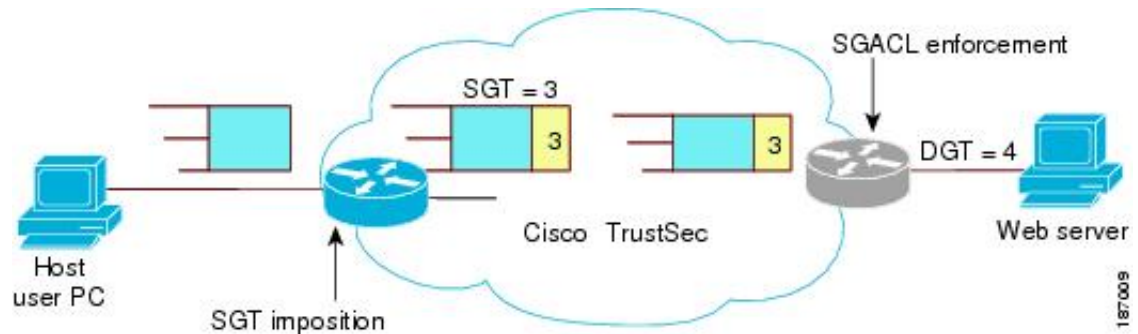
Figure 3: SGT and SGACL in a Cisco TrustSec Domain
