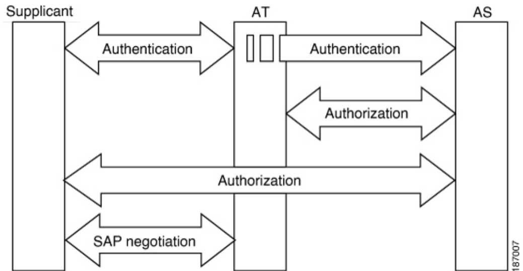
Figure 4: NDAC and SAP Negotiation
