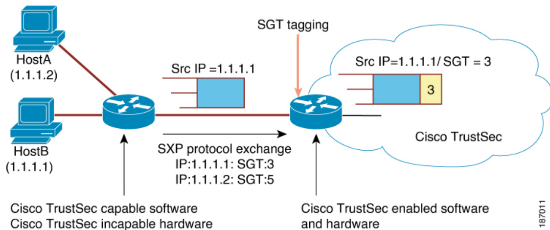
Figure 5: SXP Protocol to Propagate SGT Information
