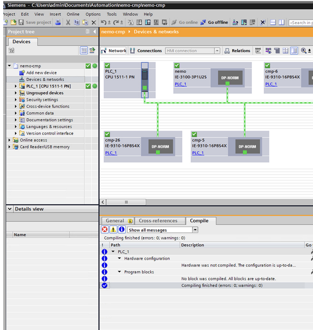
Figure 6: PROFINET MRP network configuration diagram
