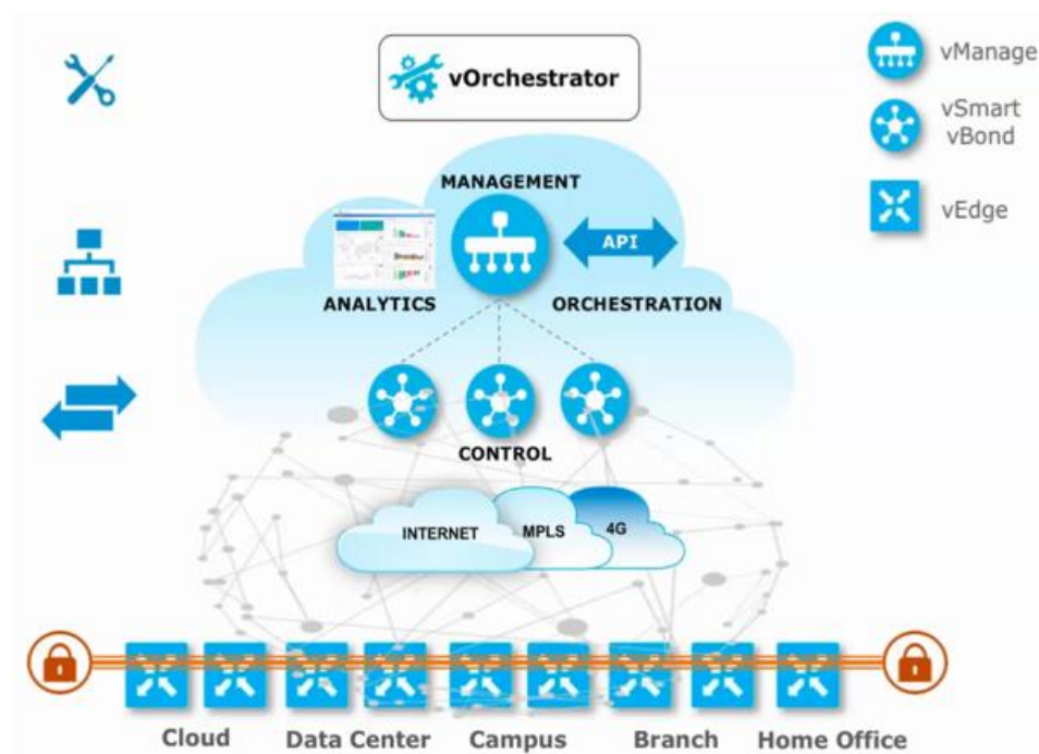
Figure 1: High level architecture of SD-WAN
