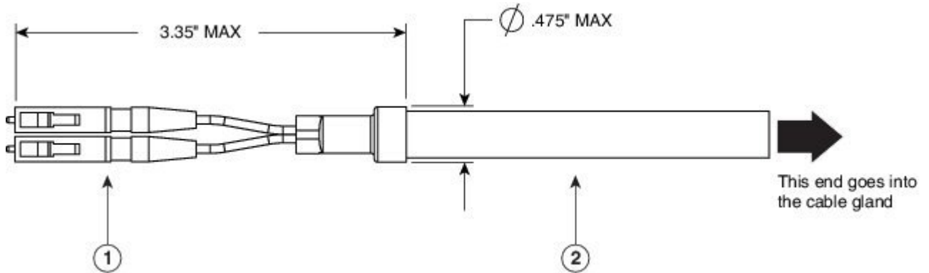
Figure 7: Duplex LC Fiber Optic Cable
