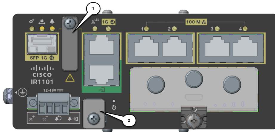
Figure 3: Cisco Catalyst IR1101 Rugged Series Router with USB covers in place
