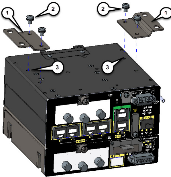
Figure 6: Mounting Brackets
