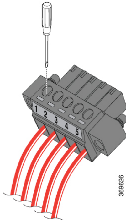
Figure 13: Alarm Connector Captive Screws
