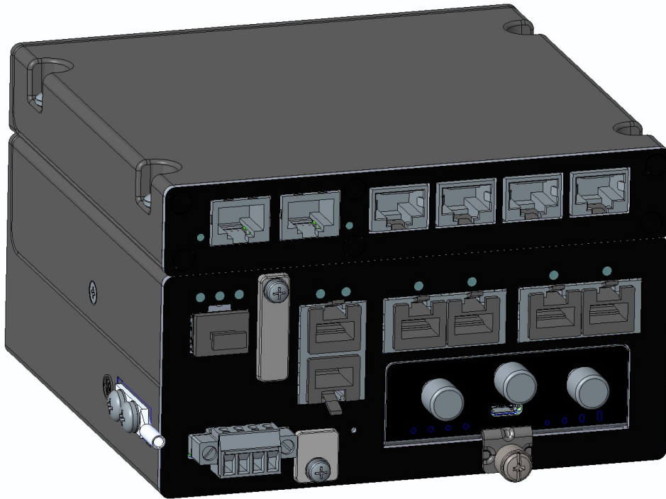
Figure 3: Completed Assembly
