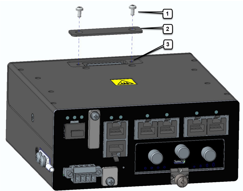
Figure 1: Protective Cover
