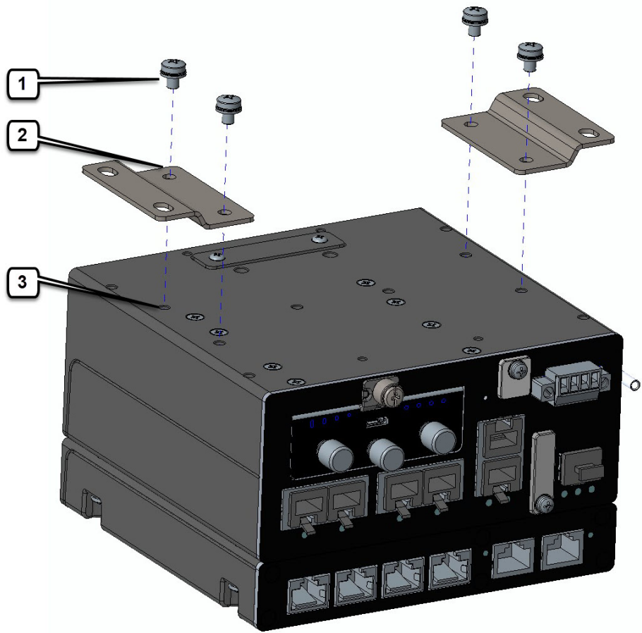
Figure 9: Mounting Brackets
