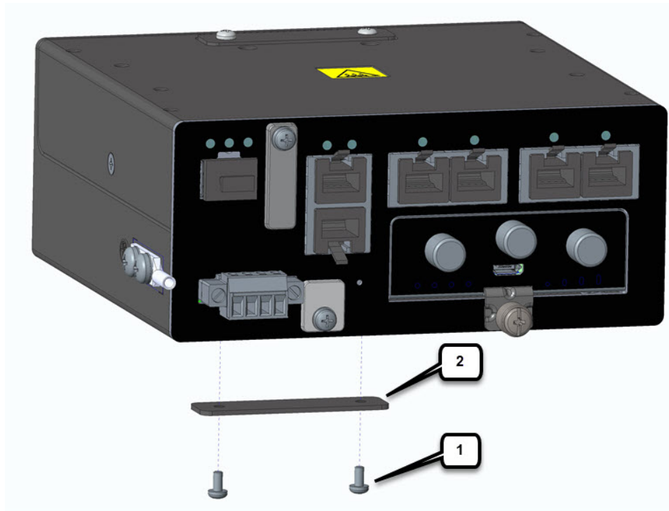
Figure 4: Protective Cover
