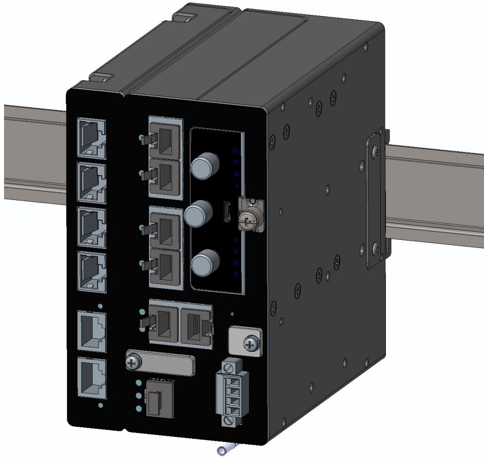
Figure 12: Device Orientation
