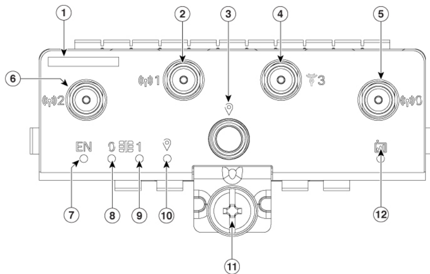
Figure 1: 5G Pluggable Interface Module - P-5GS6-GL, P-5GS6-R16SA-GL
