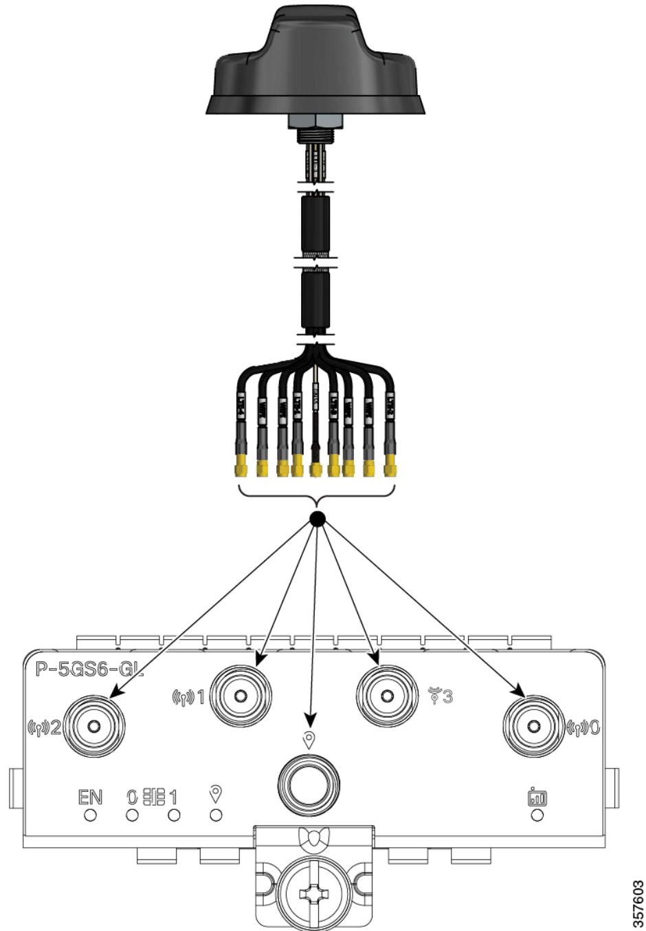
Figure 2: Attaching 5G NR Antenna (5G-ANTM-04-B) to P-5GS6-GL, P-5GS6-R16SA-GL PIM
