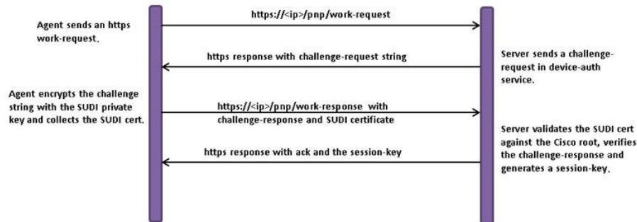
Figure 13: Message Sequence
