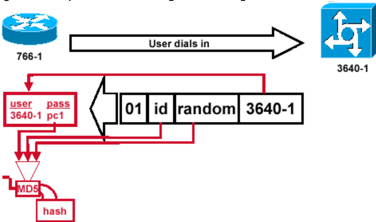
Figure 4 – Receipt and MD5 Processing of the Challenge Packet from the Peer
