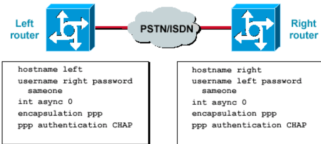
Figure 1 – Two Routers Connected Across a Network
