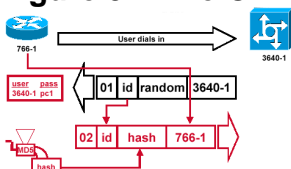
Figure 5 – The CHAP Response Packet Sent to the Authenticator is Built.
