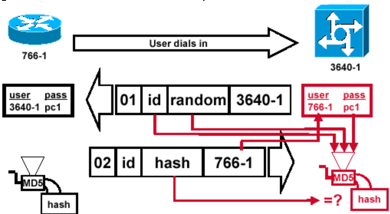
Figure 6 – The Authenticator Processes the Response Packet
