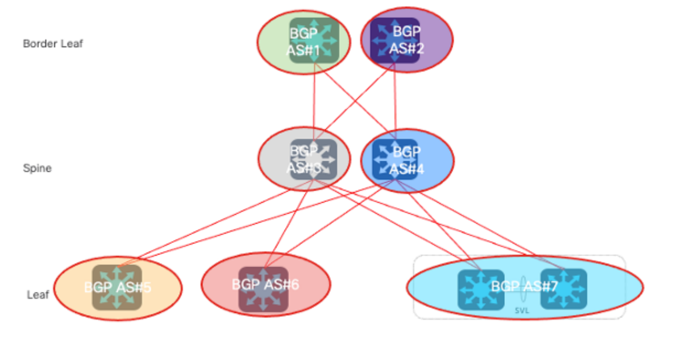
Multi-AS Model
