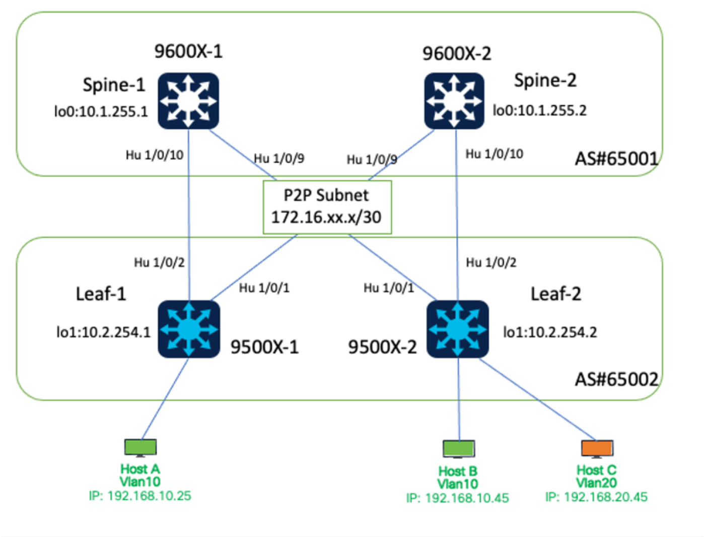
Network Diagram
