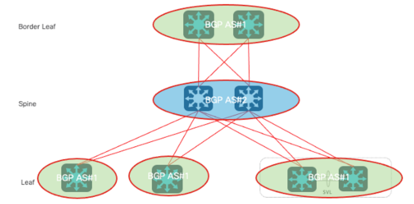
Two-AS Model
