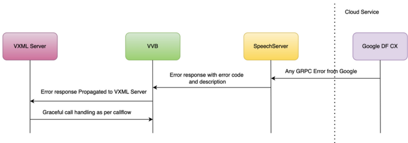
gRPC Error Propagation Flow Diagram
