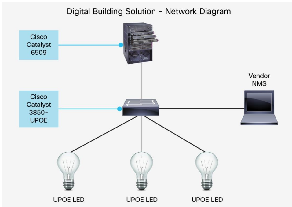
Figure 1. Digital Building Solution Connectivity to Cisco Catalyst Switches
