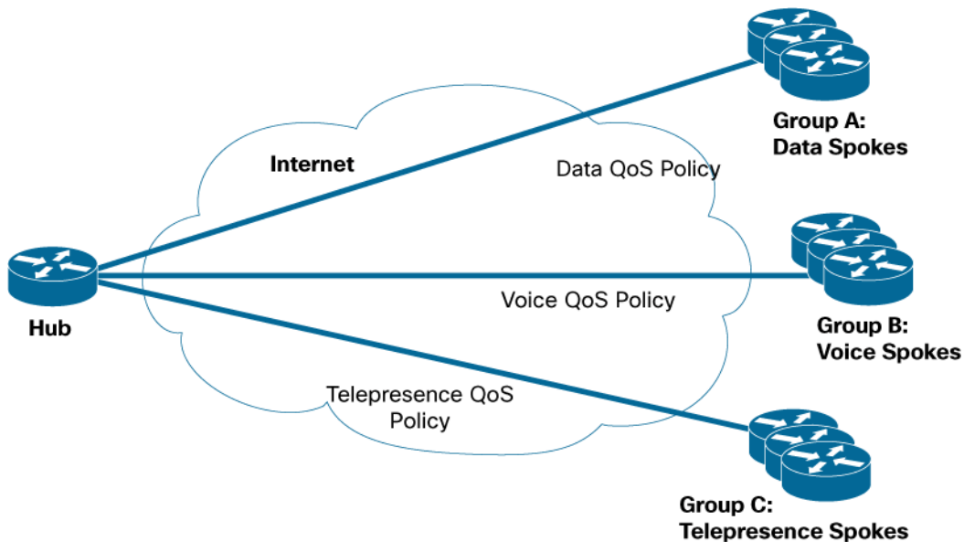
Figure 1. Cisco Virtual Office DMVPN Hub-and-Spoke Topology and Per-Tunnel QoS Setup
