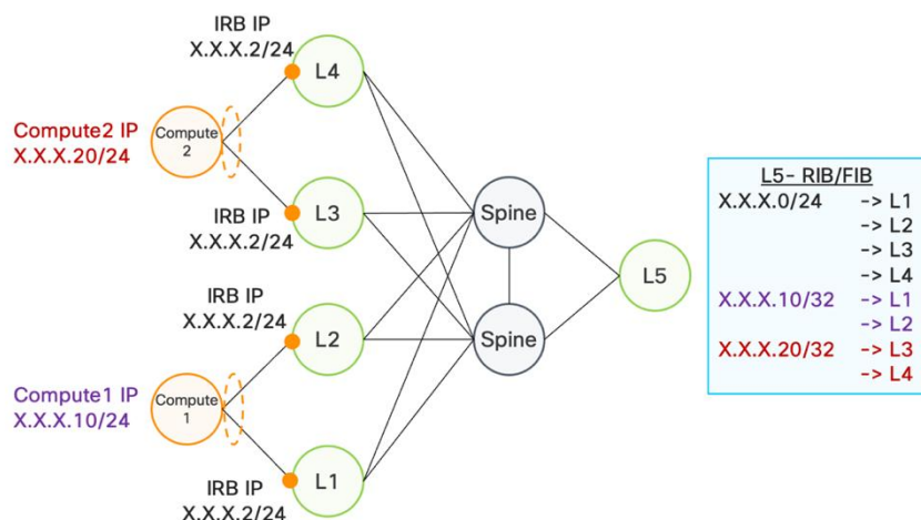
Figure 23. EVPN Host Routing
