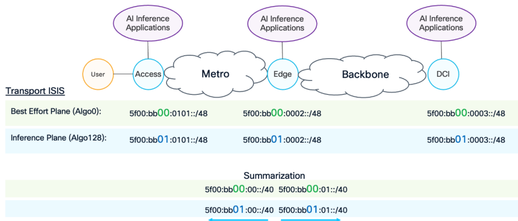
Figure 9. Multi-plane backbone design for AI Inference connectivity
