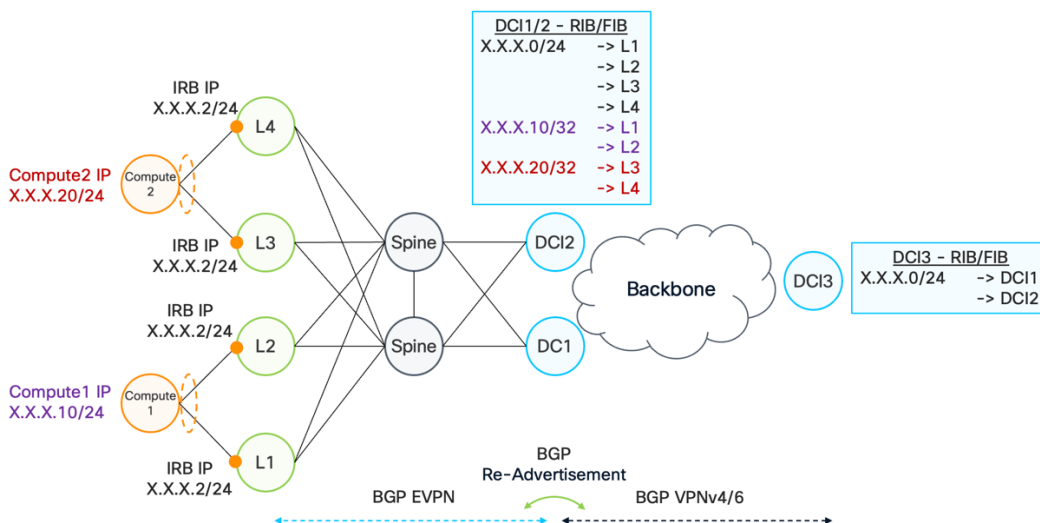
Figure 18. DCI Route Summarization
