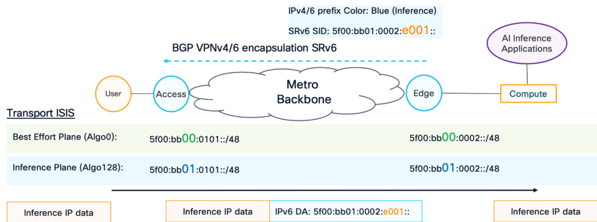
Figure 12. AI Inference cluster – Remote connectivity with Direct IP Handoff
