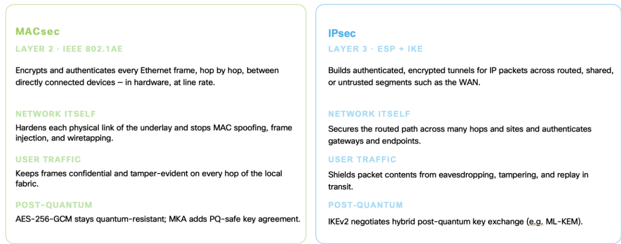
Figure 27. Securing Transport Layer
