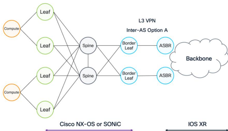
Figure 19. Border Leaf – DCI Lite
