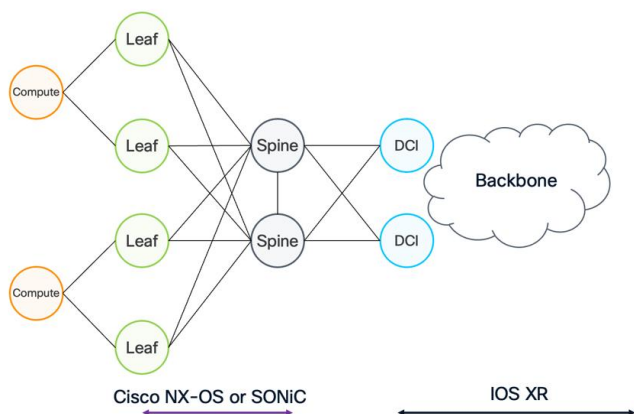
Figure 17. Backbone to Datacenter Interconnect
