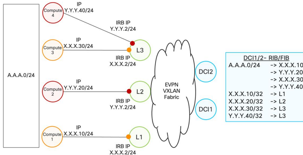
Figure 26. IP Gateway
