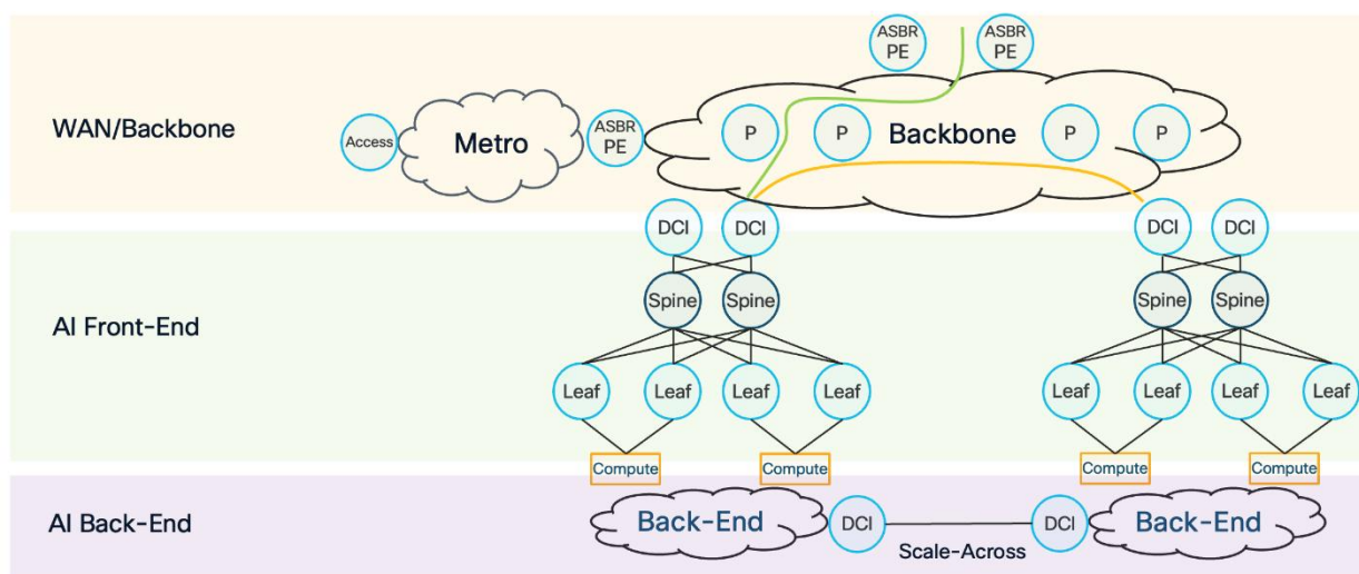
Figure 4. AI Inference Networking Layers
