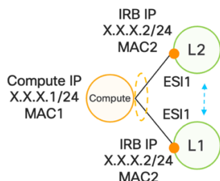
Figure 21. Distributed Anycast Gateway
