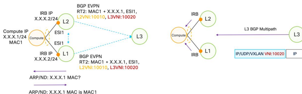
Figure 22. Mac and IP Advertisement
