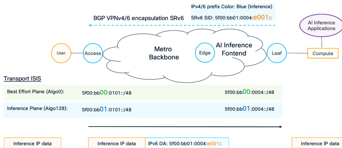
Figure 15. AI Inference cluster – External peering
