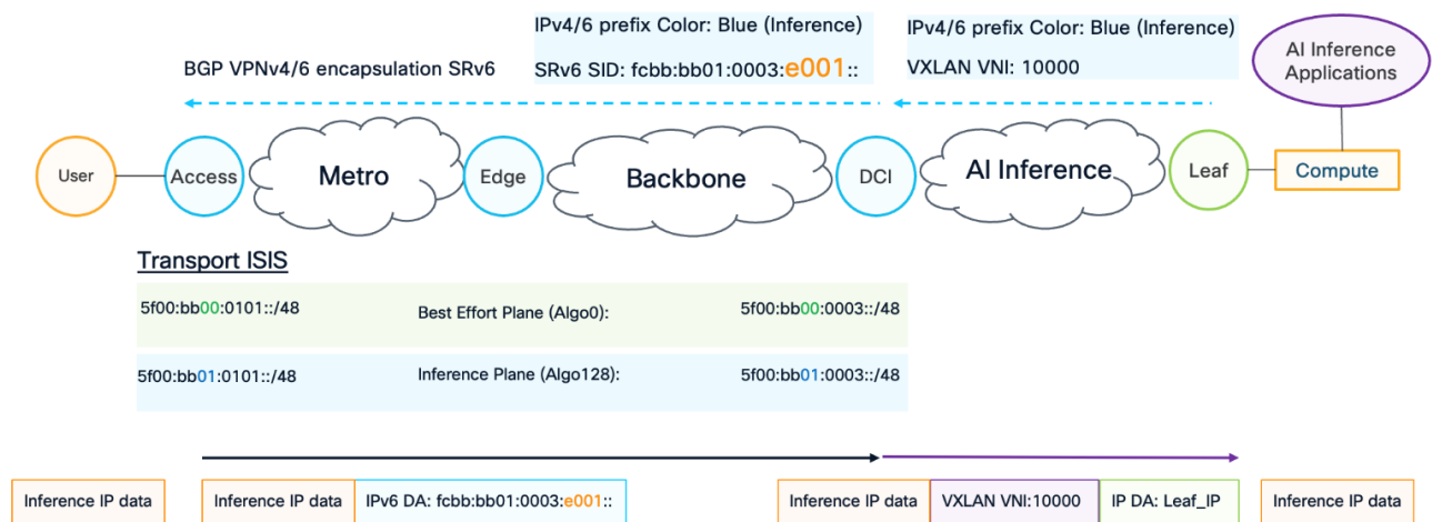
Figure 13. AI Inference cluster – AI Frontend service overlay
