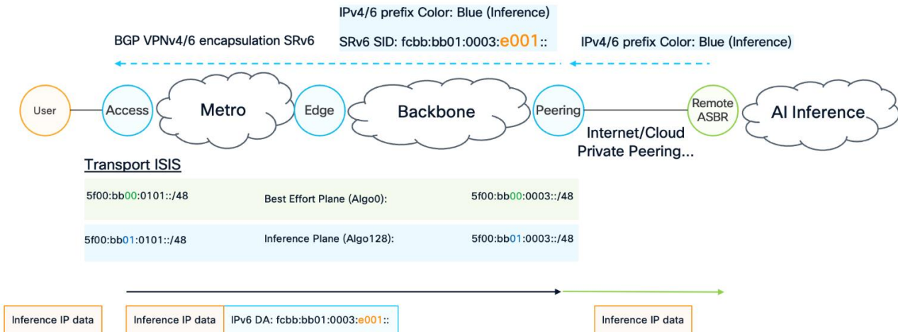
Figure 14. AI Inference cluster – External peering
