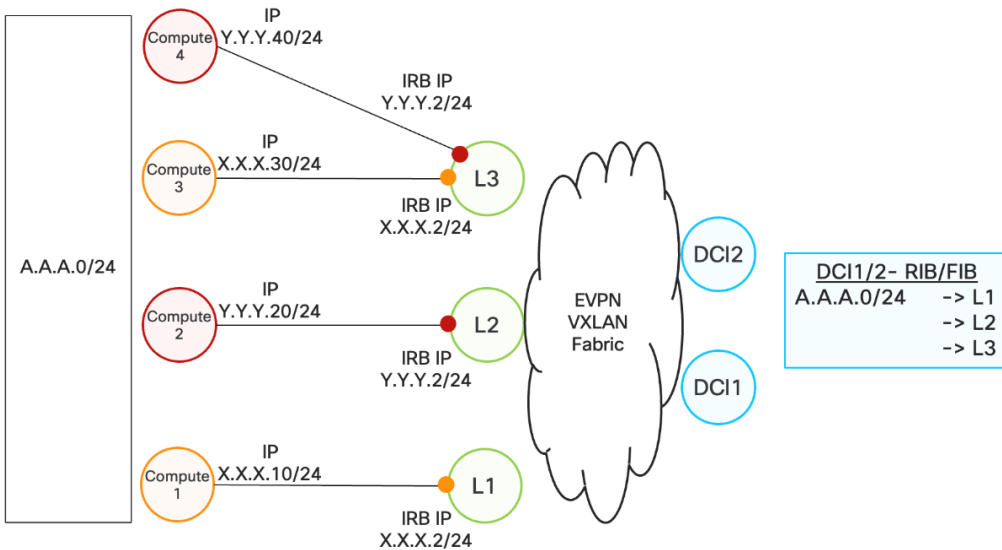
Figure 25. Weighted ECMP
