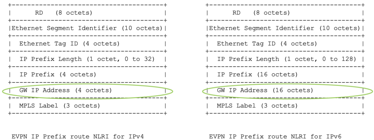
Figure 24. RT5 with IP Gateway
