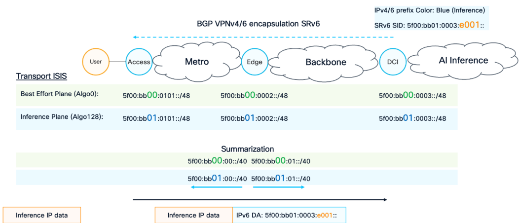
Figure 10. BGP signaling for Inference connectivity
