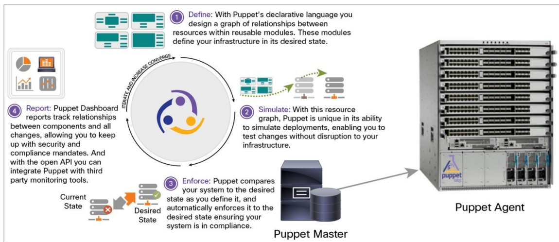
Figure 1. How Puppet Enterprise Automation Software Works
