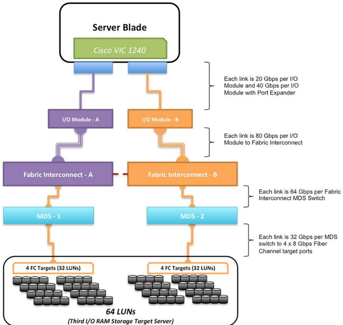
Figure 4. Network Topology
