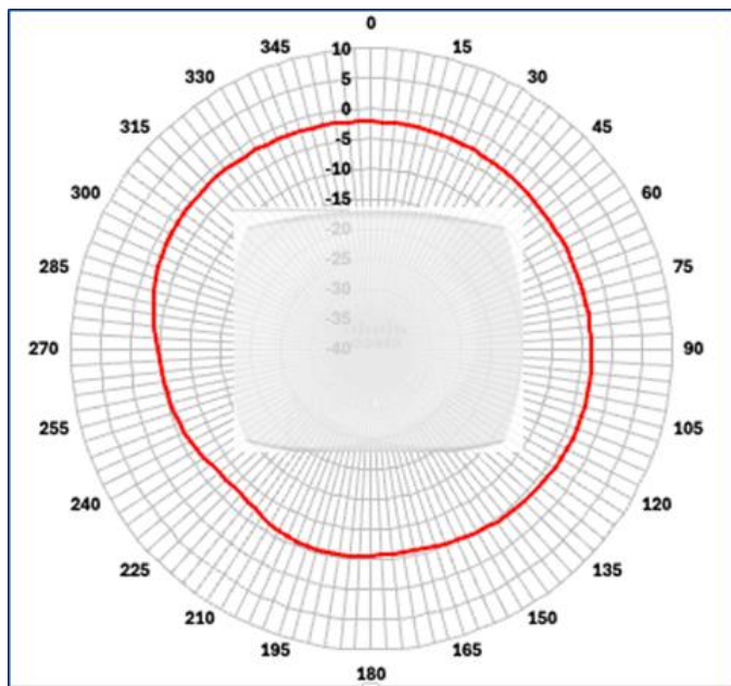
Figure 6. GNSS antenna patterns
