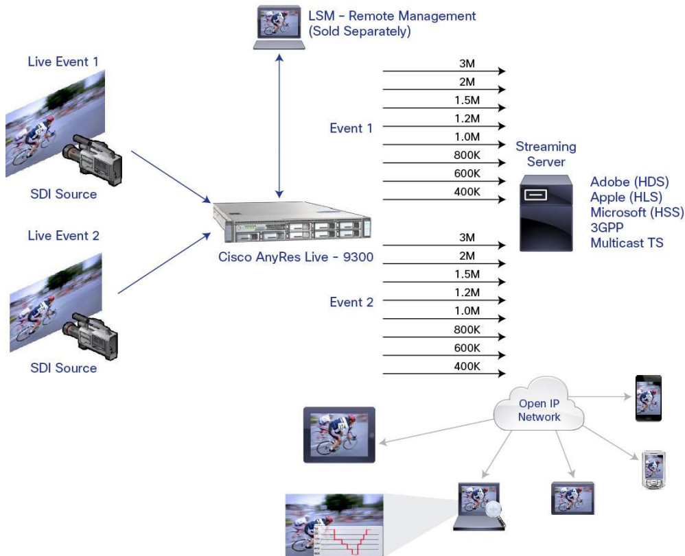
Figure 1. Cisco AnyRes Live - 9300 Workflow Example
