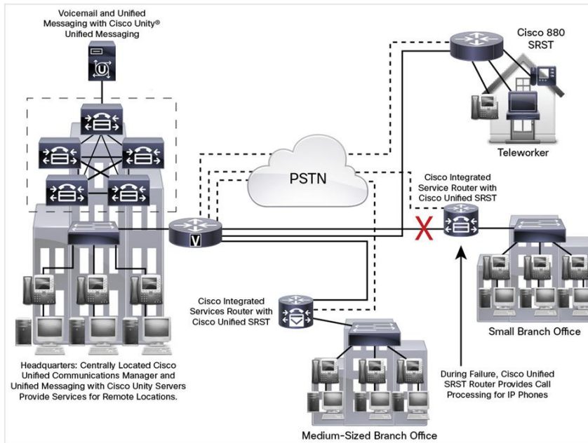
Figure 1. Centralized Cisco Unified Communications Manager Deployment with Remote Site Experiencing a WAN Failure and Cisco Integrated Services Router with Cisco Unified SRST
