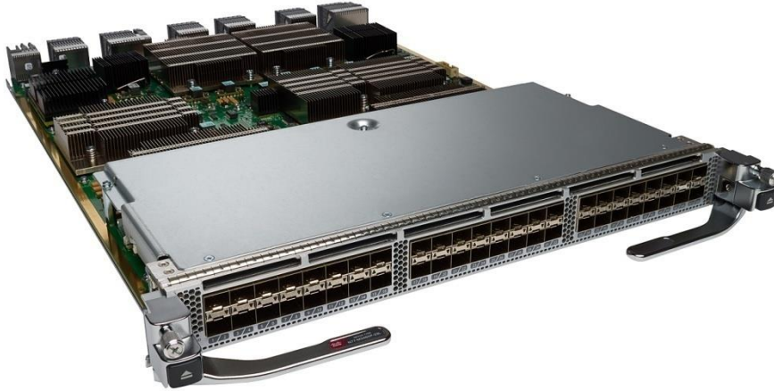
Figure 1. Cisco Nexus 7700 M3-Series 48-Port 1 and 10 Gigabit Ethernet Module
