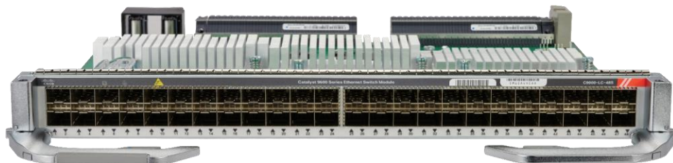
Figure 5. Cisco Catalyst 9600 Series 48-Port 1GE Line Card (C9600-LC-48S)
