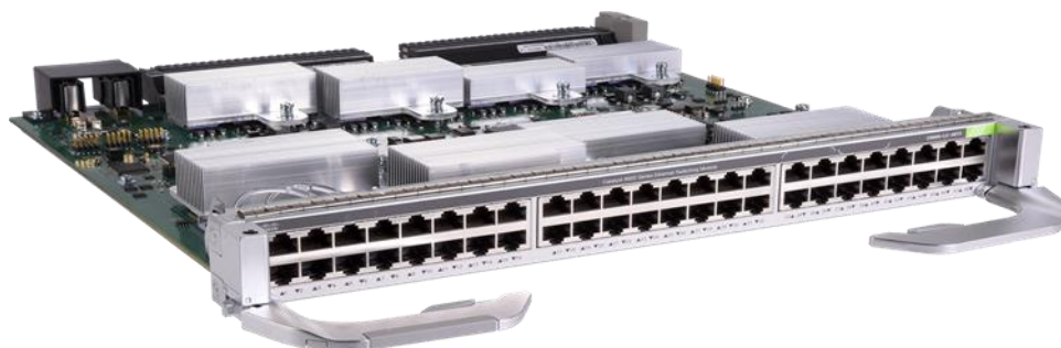
Figure 6. Cisco Catalyst 9600 48-port RJ45 Copper - 10GE/5GE/2.5GE/1GE/100Mbps/10Mbps multigigabit Line Card (C9600-LC-48TX)
