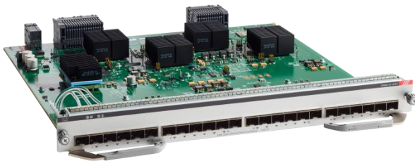
Figure 3. C9400-LC-24XS Cisco Catalyst 9400 Series 24-Port 10 Gigabit Ethernet (SFP+)
