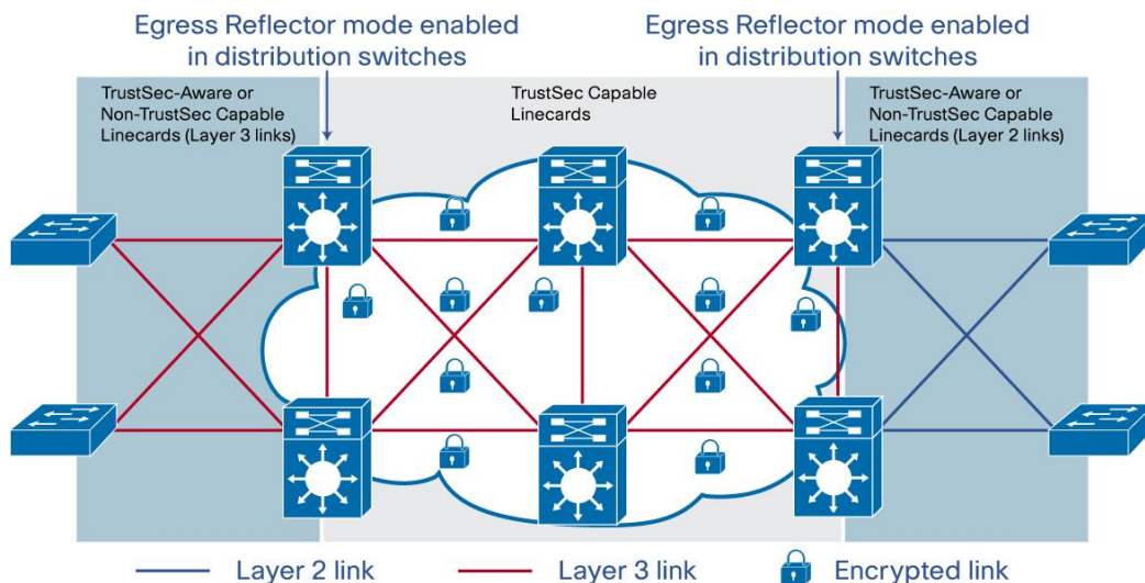
Figure 4. Egress Reflection Mode Use Case
