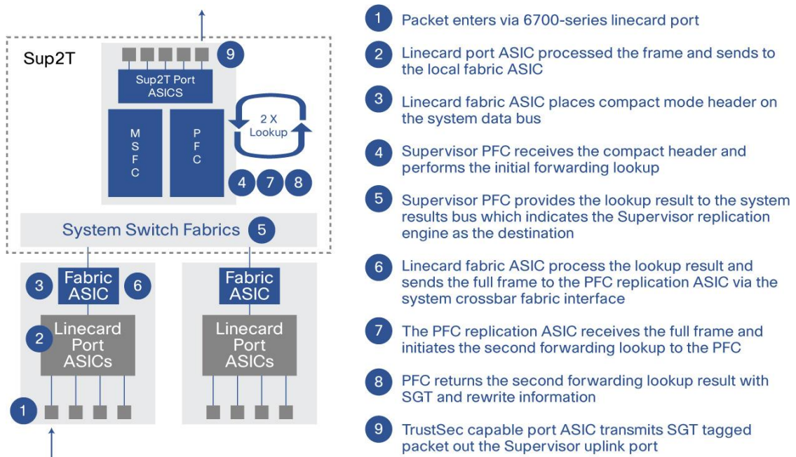
Figure 6. Egress Reflection Mode Packet Forwarding Example
