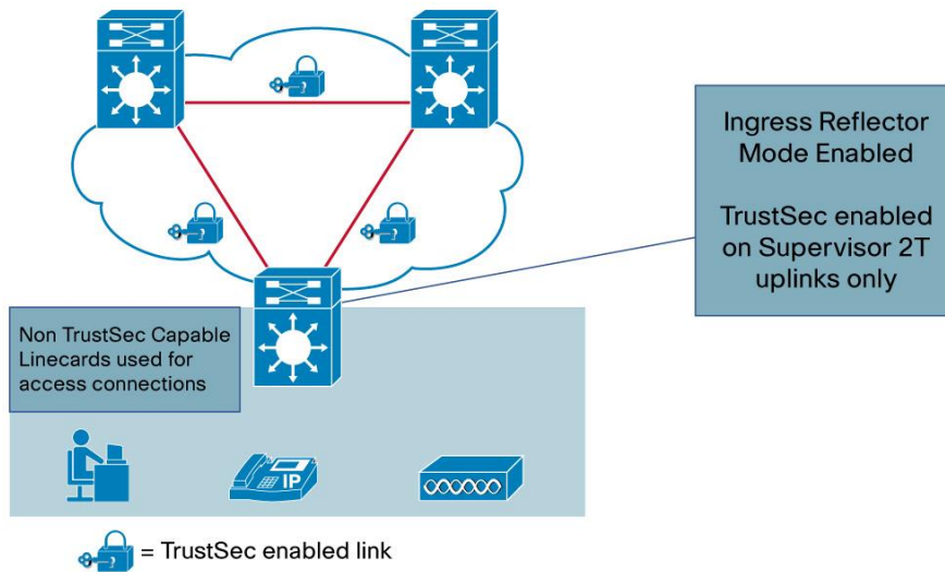
Figure 1. Ingress Reflector Mode Use Case
