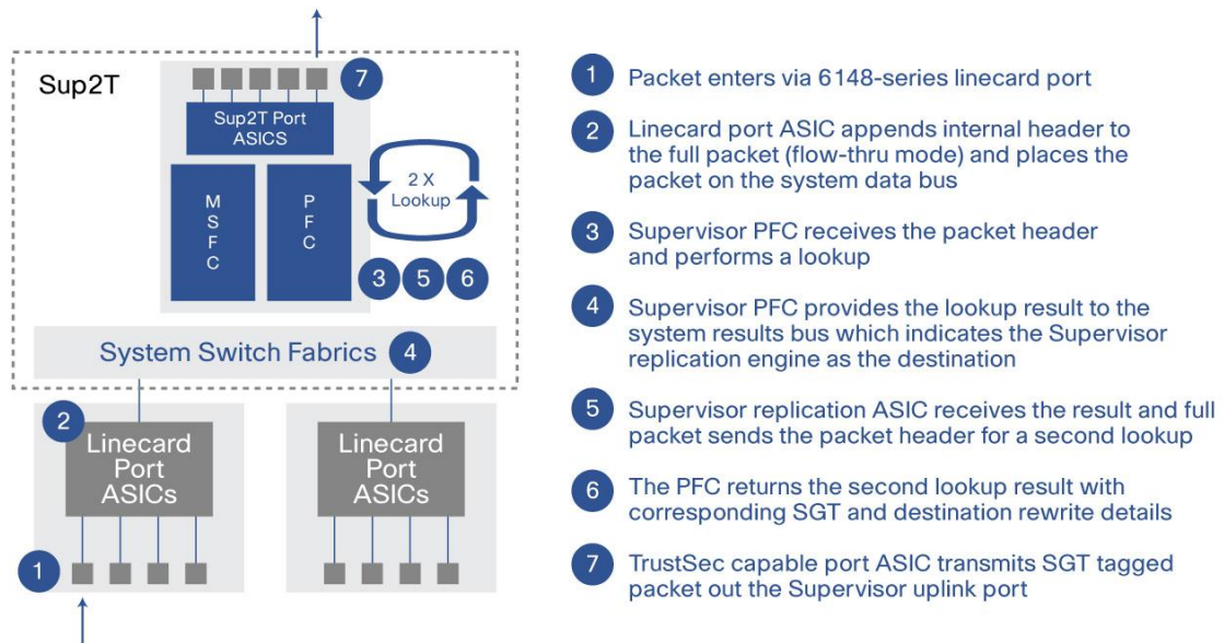
Figure 3. Ingress Reflector Mode Packet Forwarding Example
