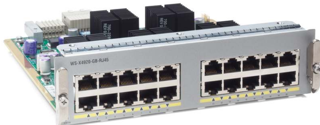
Figure 3. 4-port wirespeed 10GbE (X2) half card
