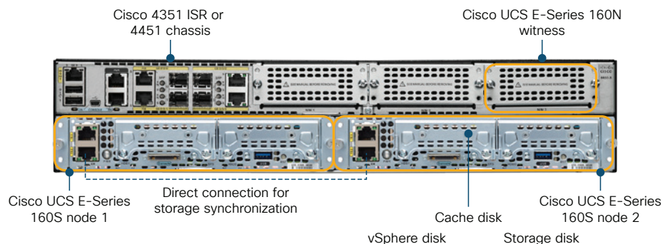
Figure 1 Cisco UCS E-Series 160S nodes in a single-wide Cisco 4000 Series ISR
