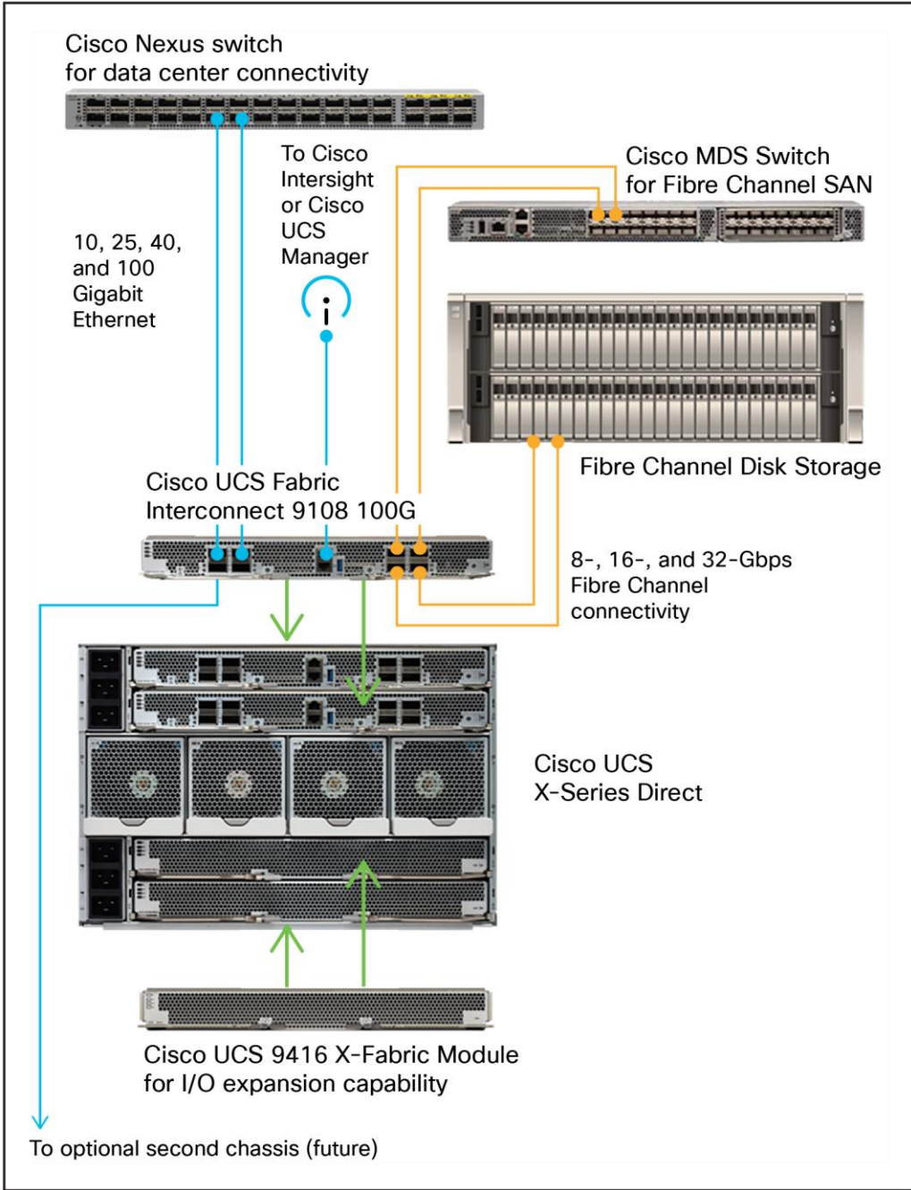
Figure 1. Cisco UCS X-Series Direct architectural options
