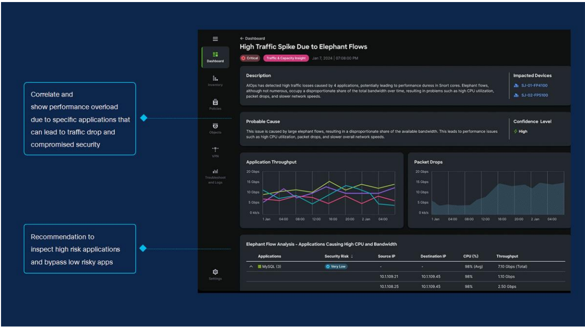
Figure 3. Predictive insights with AIOps
