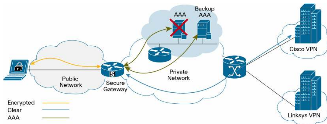
Figure 1. Cisco IOS SSL VPN Topology with Redundant AAA Servers
