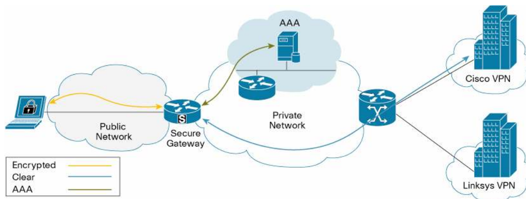
Figure 1. Basic Cisco IOS SSL VPN Topology with AAA Server
