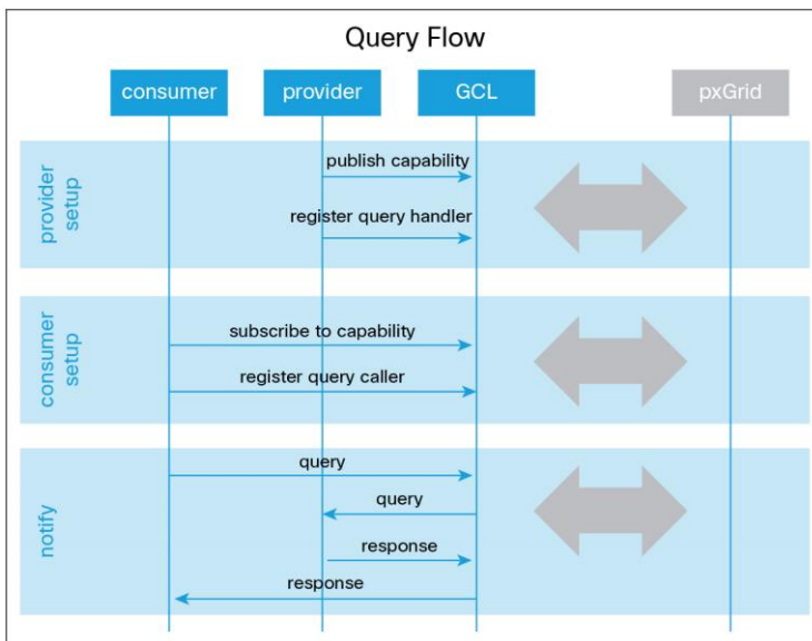
Figure 6. Query Flow
