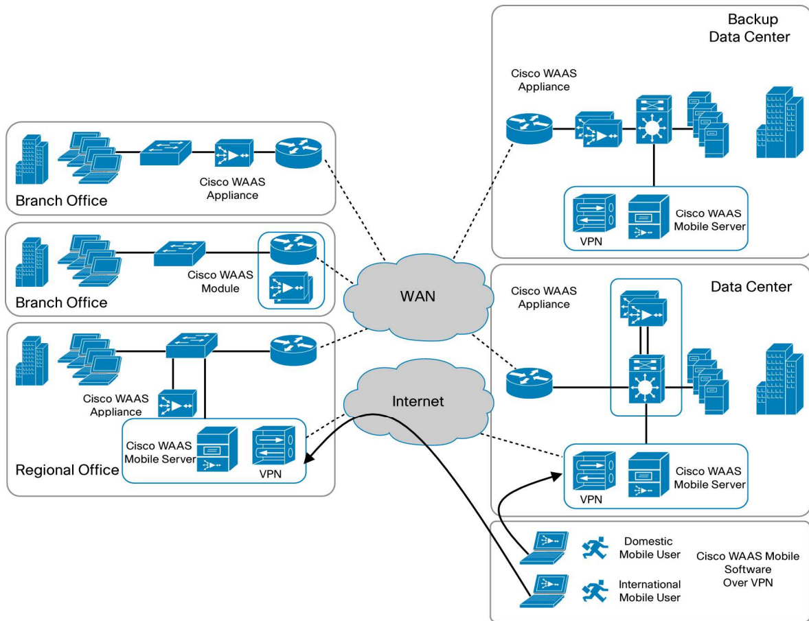
Figure 1. Cisco WAAS Deployment Architecture
