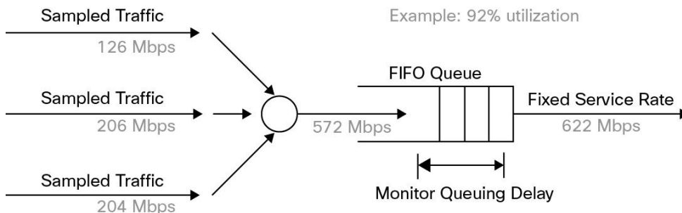
Figure 4. Queuing Simulation
