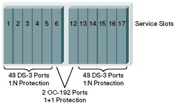
Cisco ONS 15454 Configuration with 12-Port DS-3/EC-1 Card
