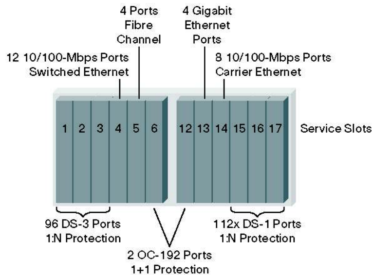
Cisco ONS 15454 Configuration with 48-Port DS-3/EC-1 Card
