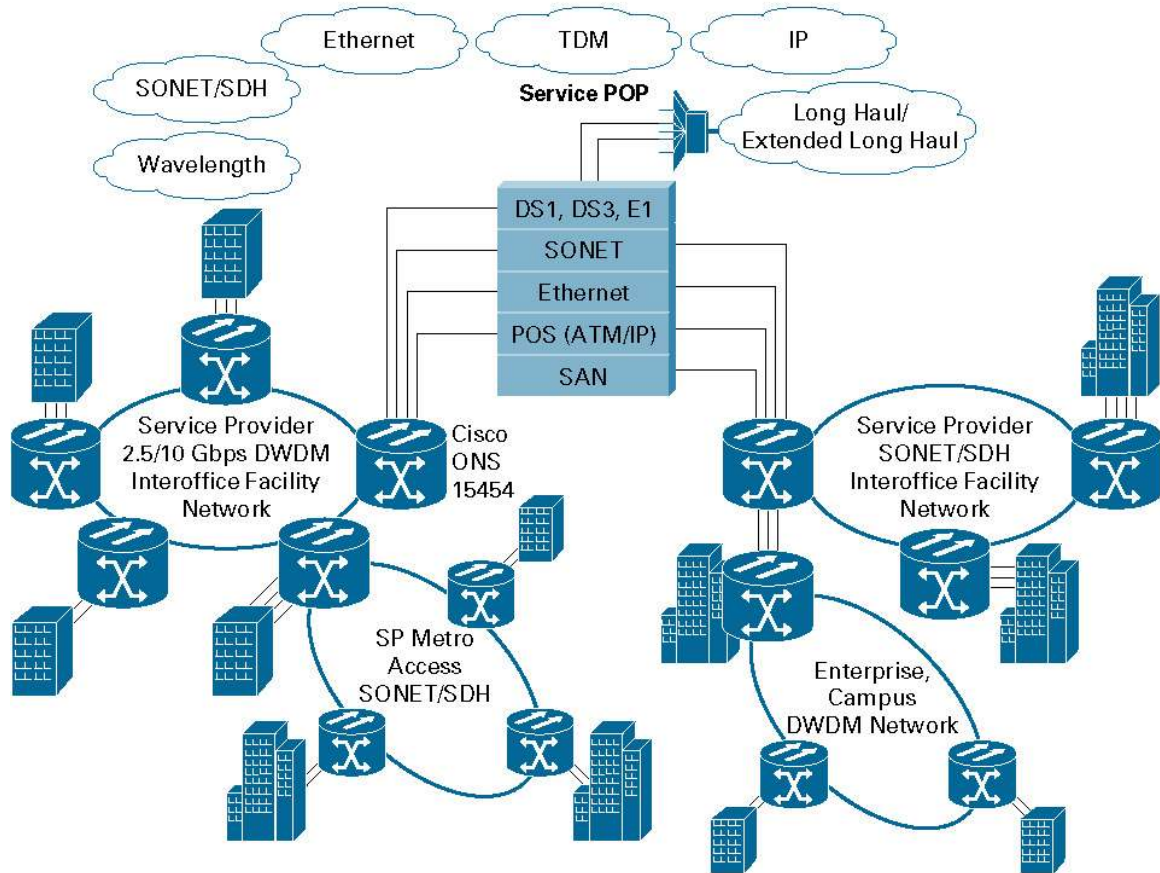
Figure 3. Metropolitan/Regional Network
