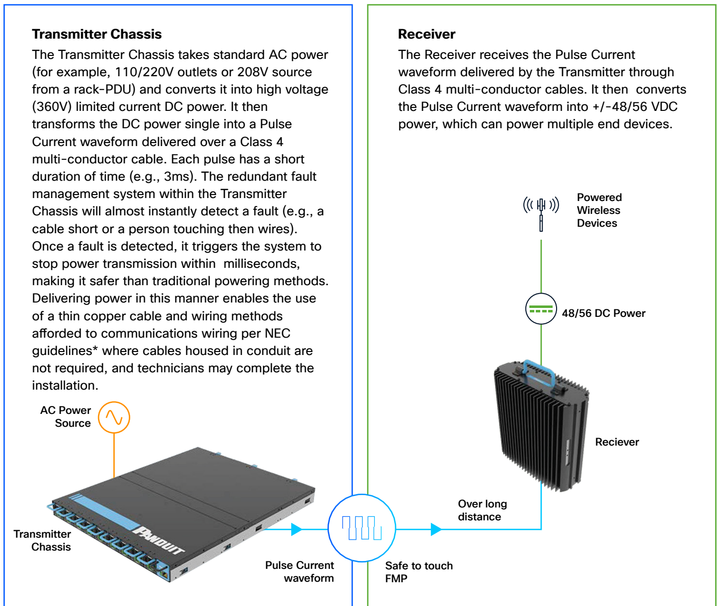
Figure 44. The Panduit FMPS at a glance
