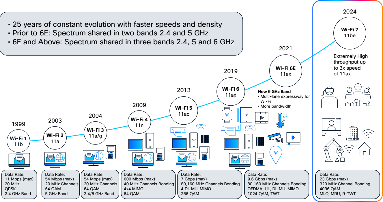
Figure 6. Wi-Fi evolution
