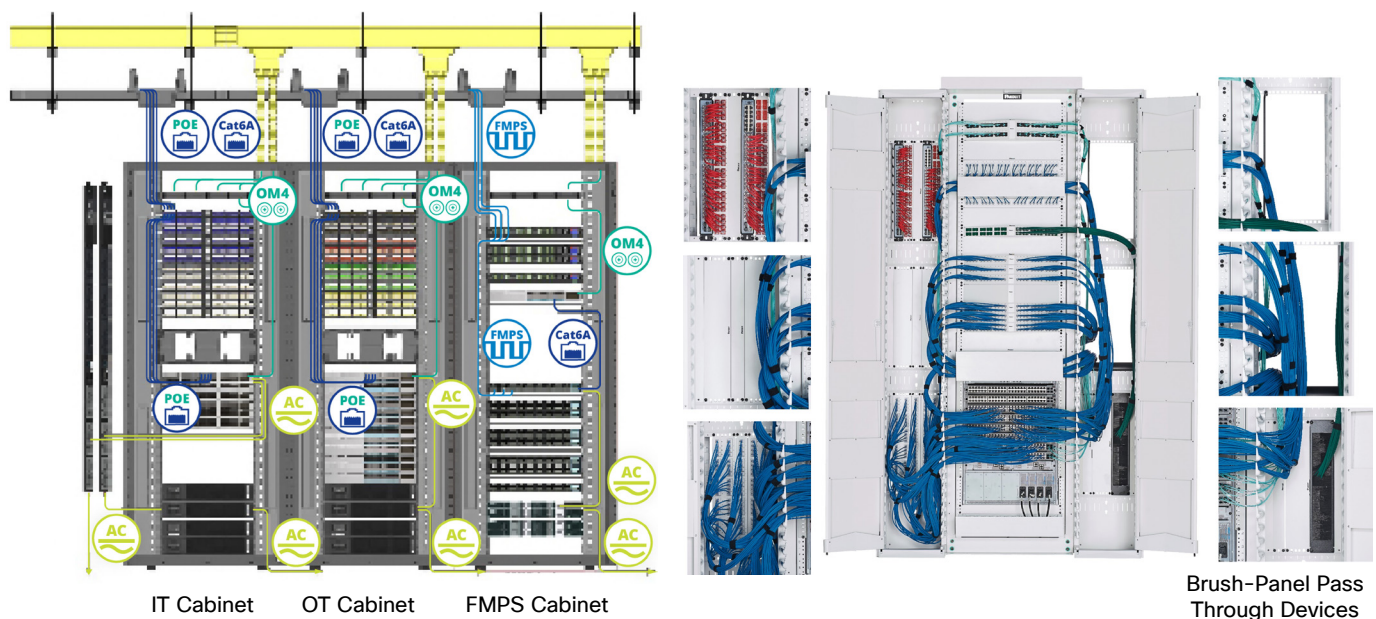
Figure 35. A telecommunications room schematic and 4-post rack
