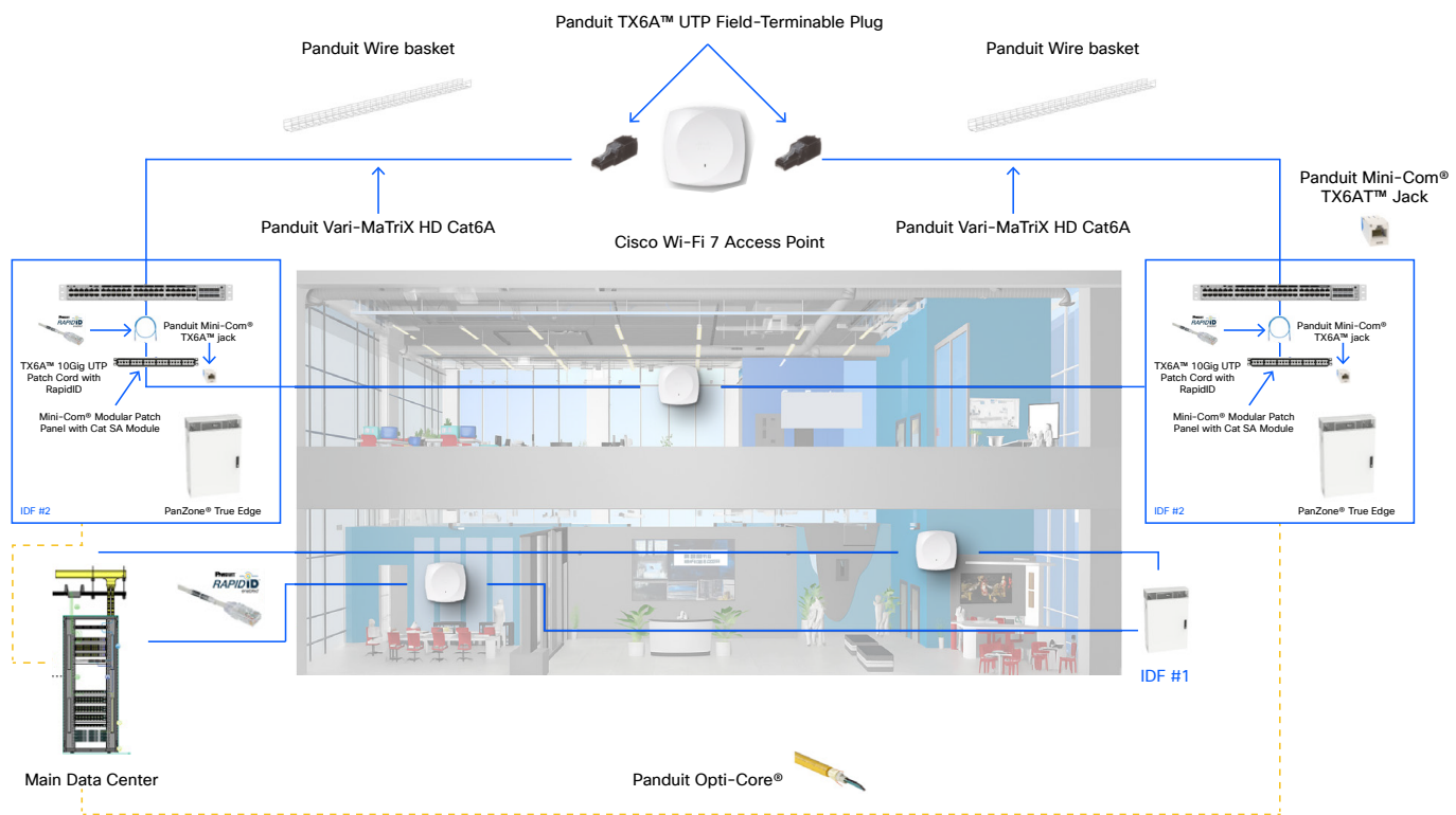
Figure 41. Smart building architecture for Wi-Fi 7 between Cisco and Panduit
