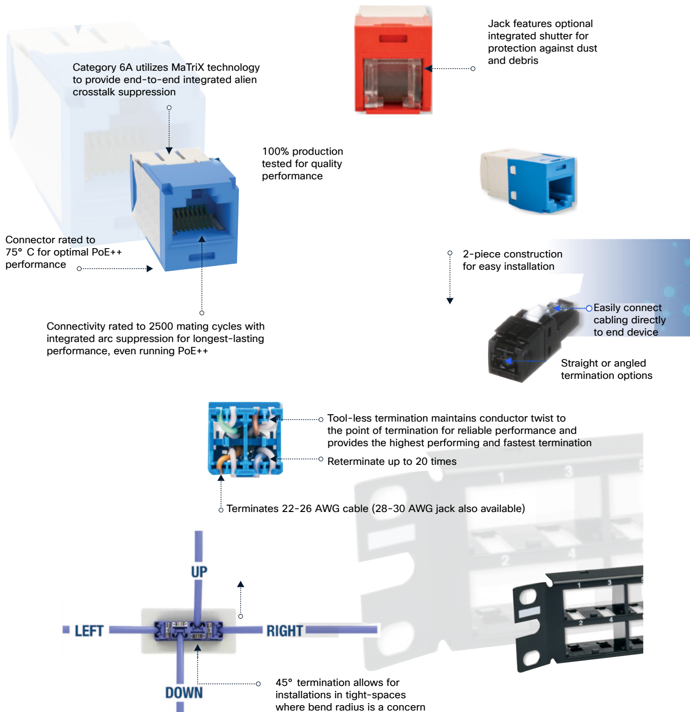
Figure 33. This image illustrates the assembly and cable management of a modular network connectivity system
