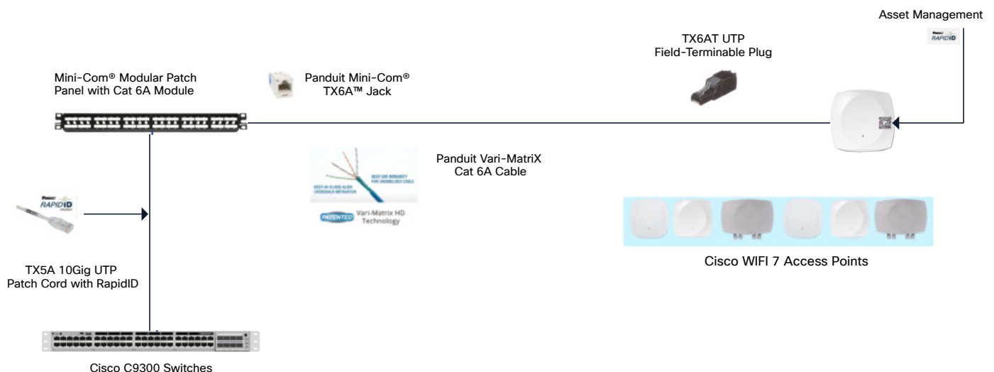
Figure 40. End to End WiFi-7 readiness
