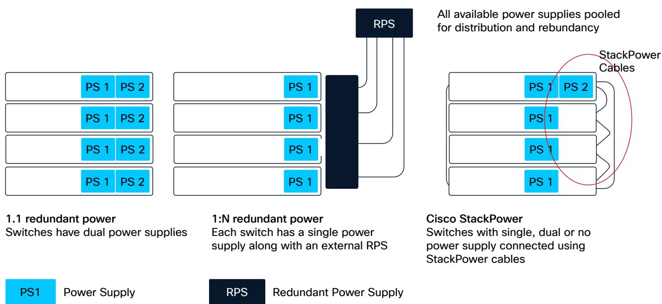
Figure 21. Strategies for power sharing and power redundancy
