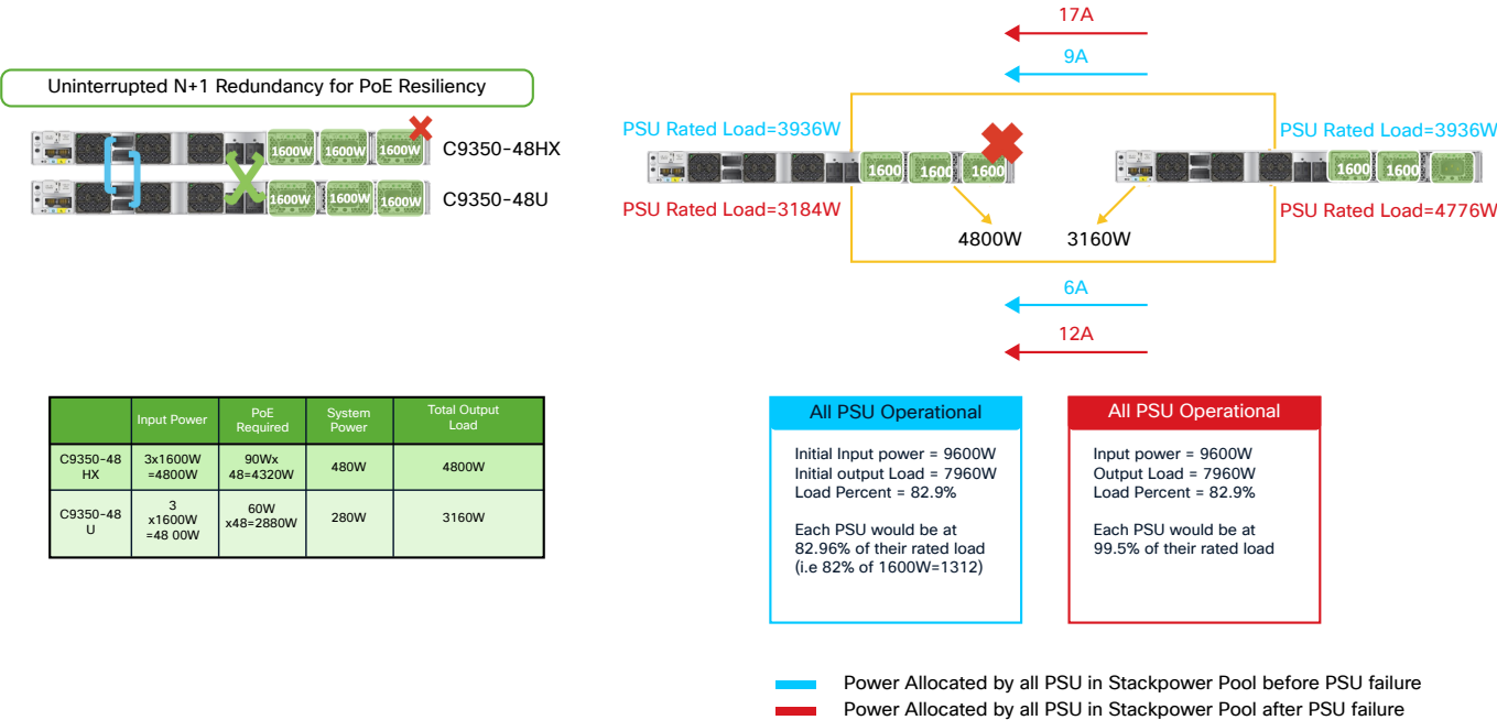
Figure 22. new StackPower+ example
