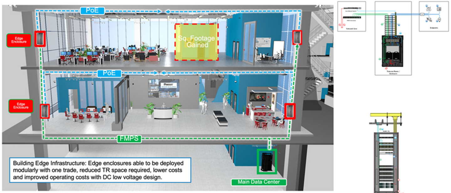
Figure 37. Edge Architecture for Telecommunications Rooms
