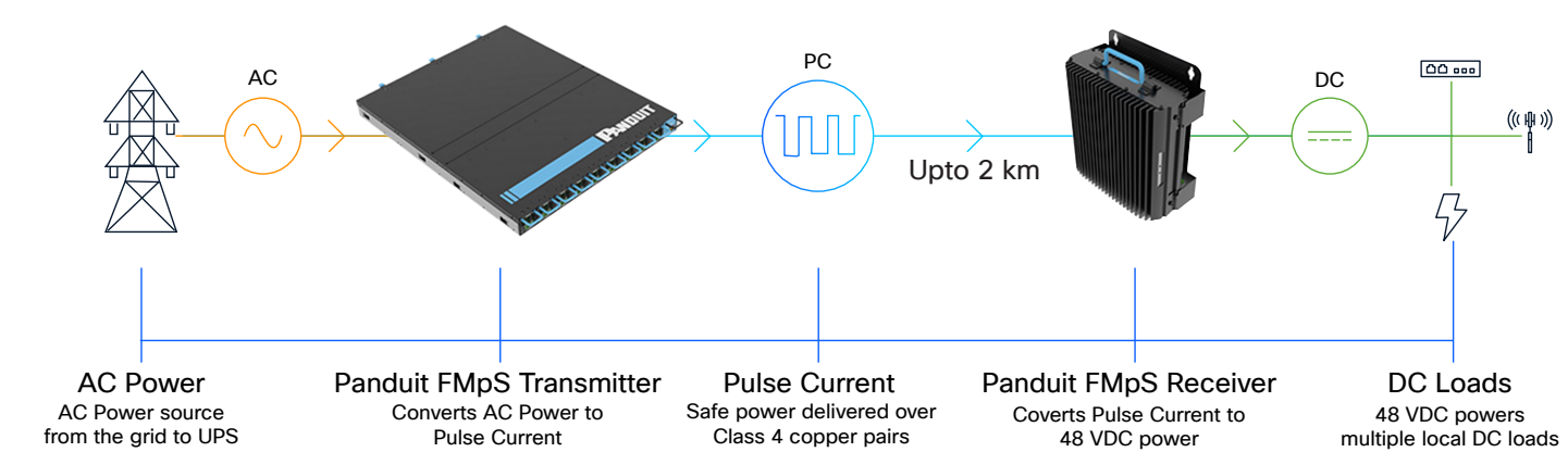
Figure 43. Panduit Fault Managed Power System
