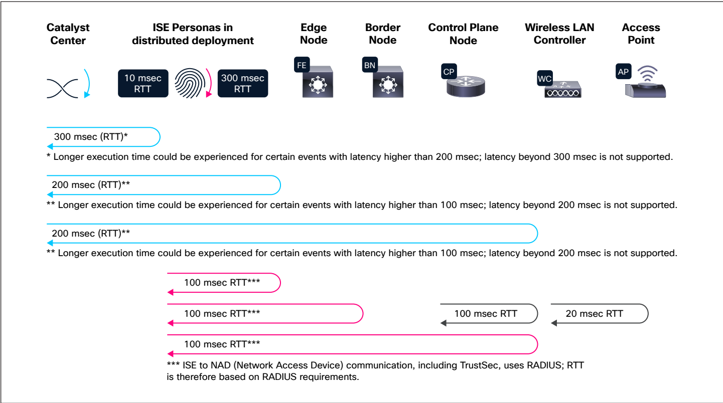
Figure 1. Maximum latency supported, roundtrip time
