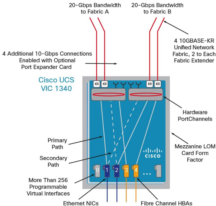
Figure 2. Cisco UCS VIC 1340 Architecture
