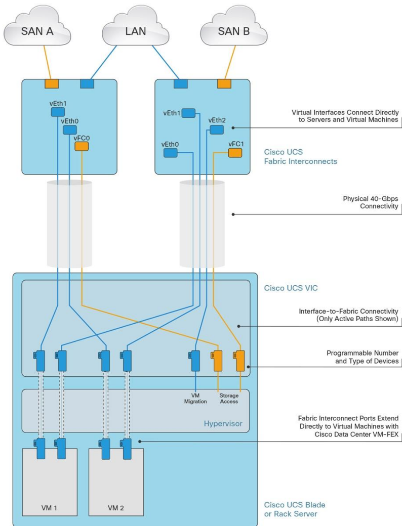
Figure 3. Cisco Data Center VM-FEX with Cisco UCS VIC 1340
