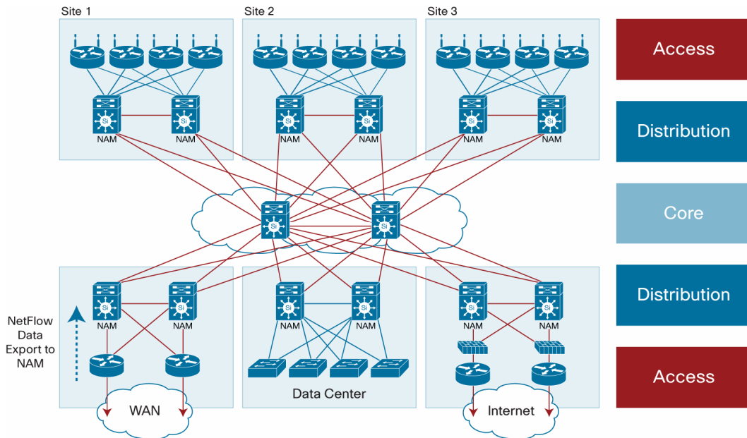
Figure 9. Deploying Cisco NAMs for Performance Monitoring in the Campus Network
