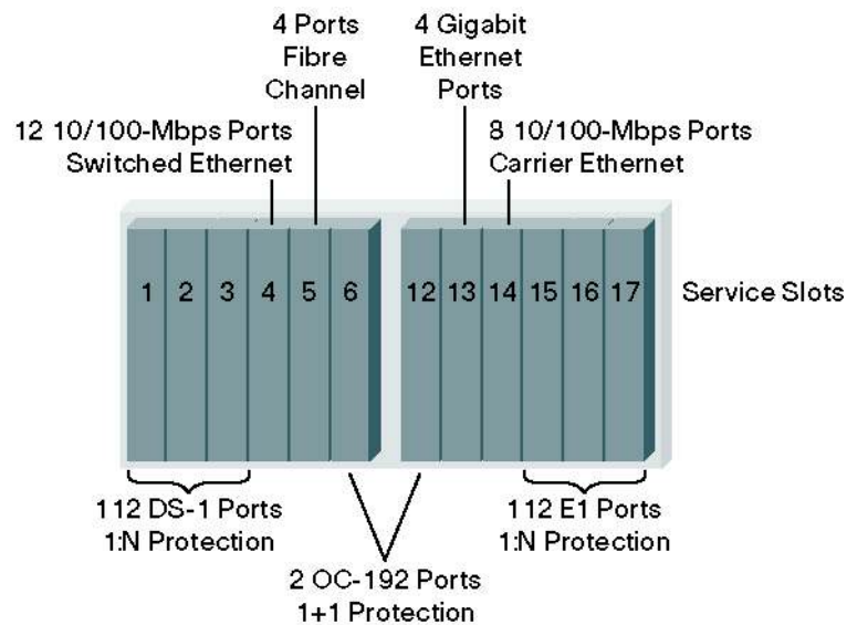
Figure 5 Cisco ONS 15454 Configuration with 56-port DS-1/E1 Card
